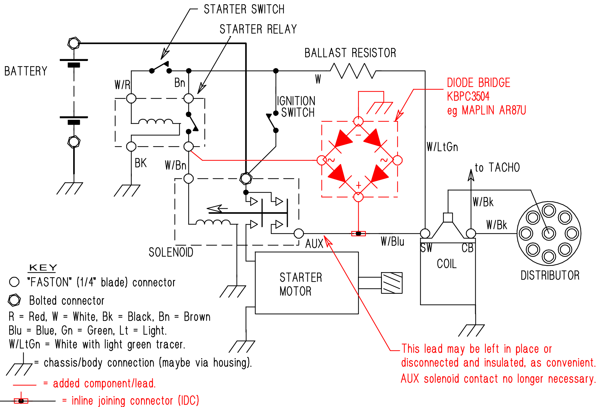
MODIFIED V8 STARTER AND IGNITION CIRCUIT
