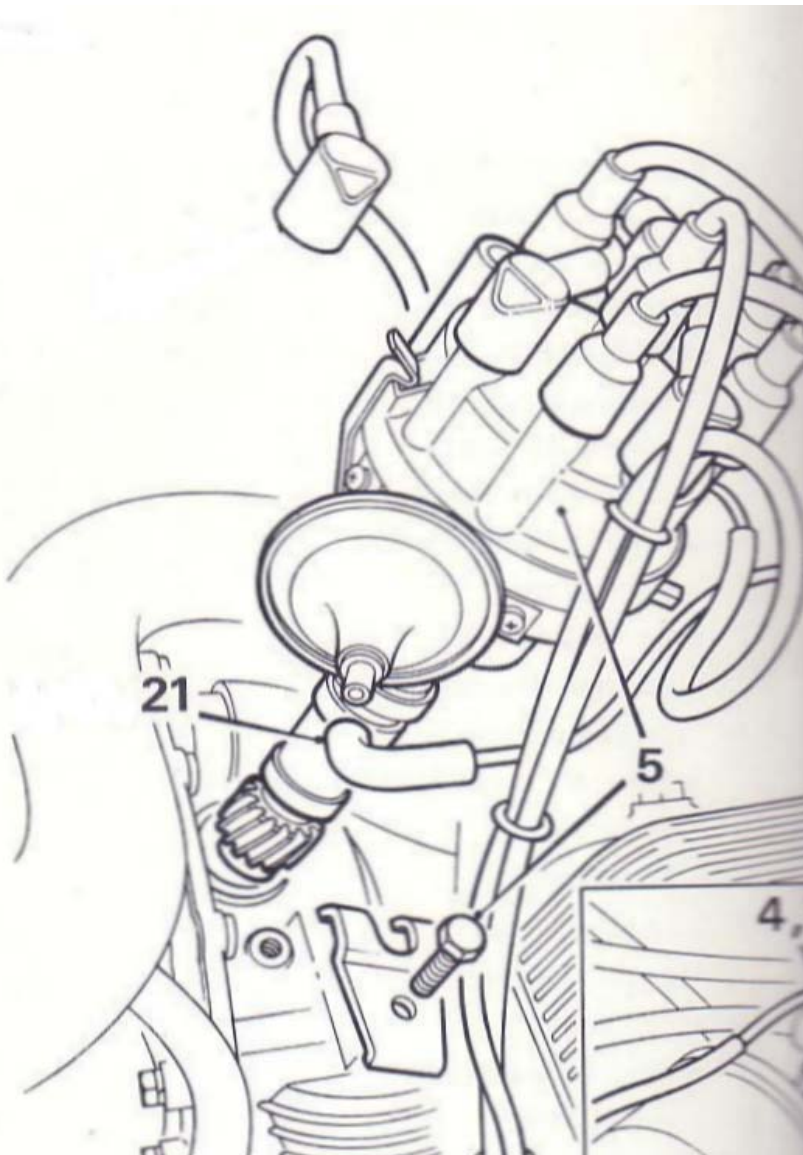
Item 21 above: vacuum pipe connects to the distributor MGBGTV8 Supplement AKD8468 Issue 1 page 86.35.20 Sheet 1
