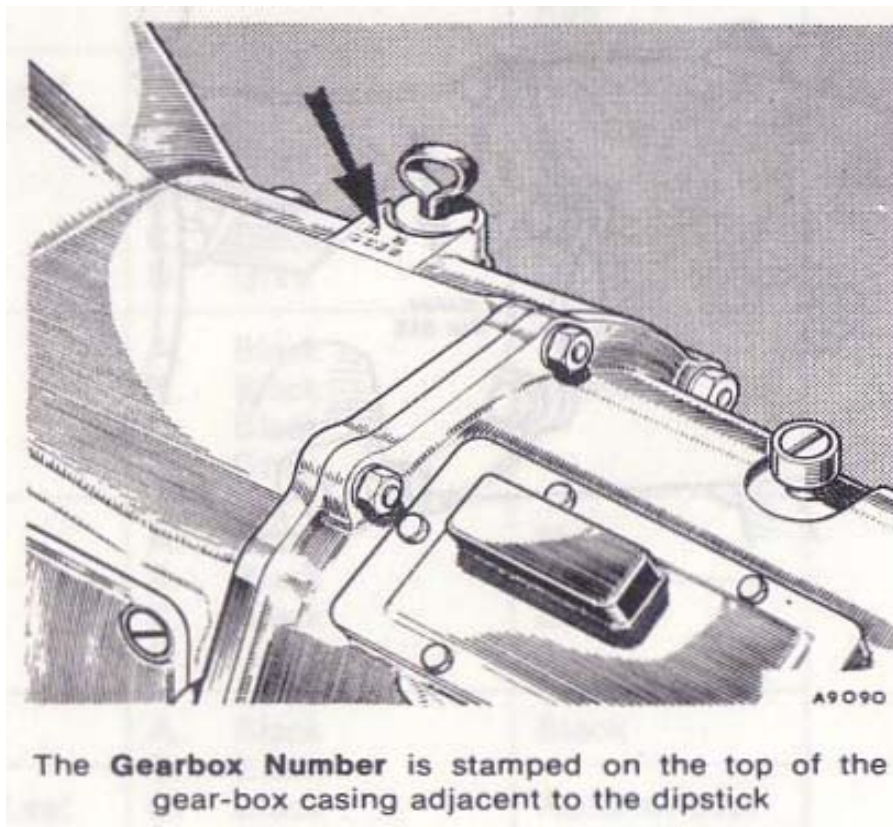
MGB gearbox – note the dipstick on the side
