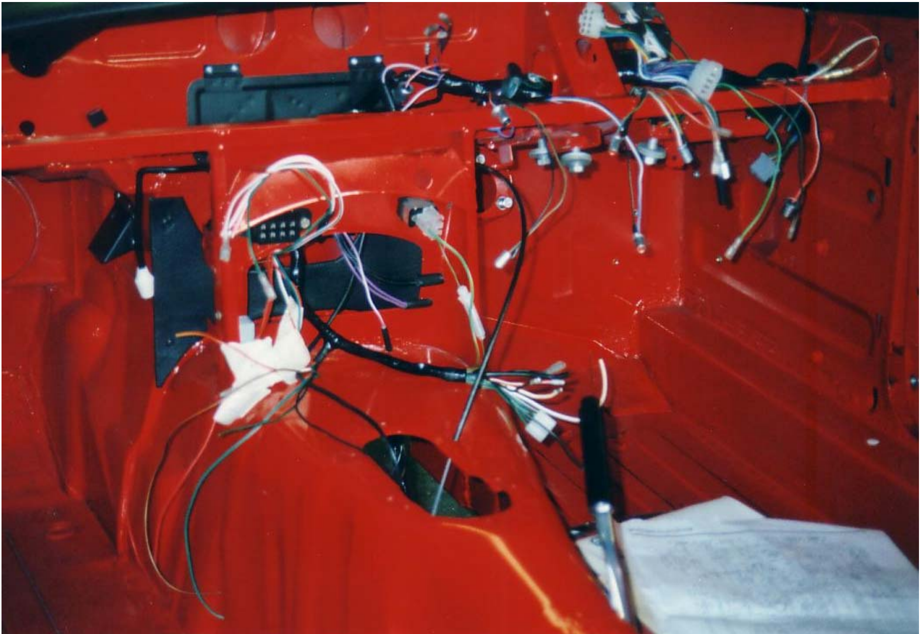
Interior wiring loom and additional fuse board fitted.
