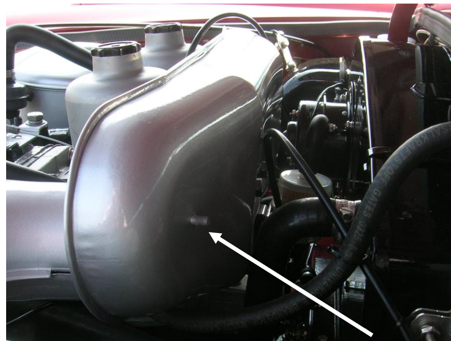
Exposed thread of a bolt through the airbox – it needs a nut and serrated washer!
